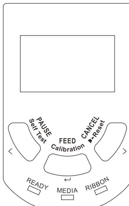
Figure 3-1 Front Panel
