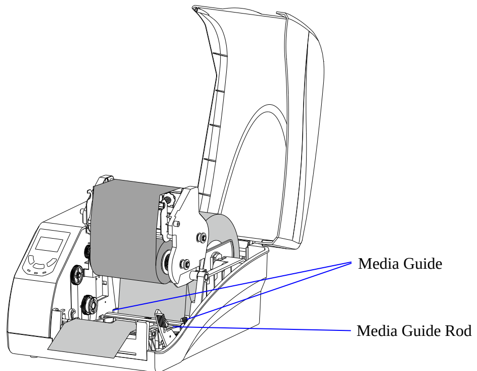
Figure 2-12 Load the Media
