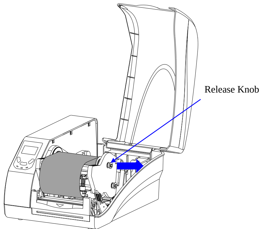
Figure 2-9 Place the Core on Ribbon Take-up
