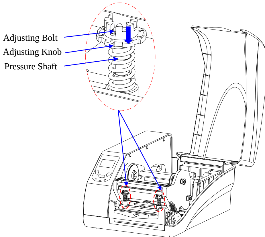
Figure 3-3 Printhead Pressure Adjustment
