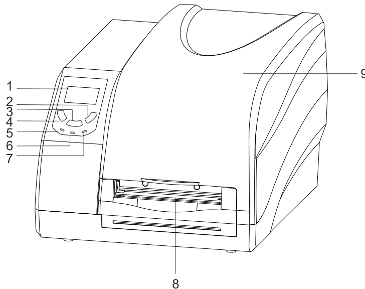
Figure 2-1 Front View
