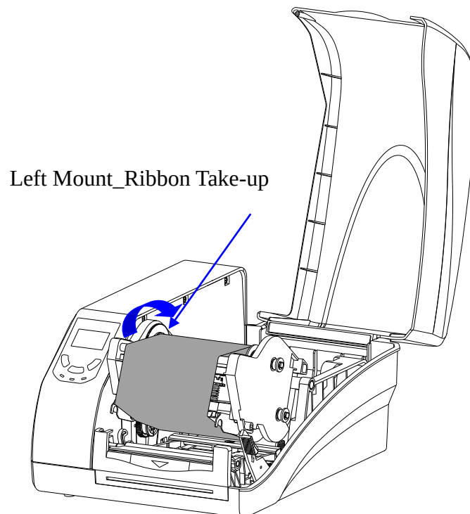
Figure 2-10 Ribbon Roll loaded
